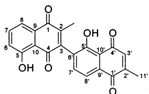
chitranone ( 3 )
